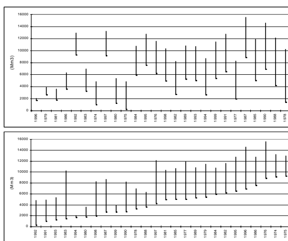
FIGURE 13: ACTIVE STORAGE DRAWDOWN BETWEEN THE 1 ST OF JANUARY AND JULY, CLASSIFIED ACCORDING TO THE MAGNITUDE OF DRAWDOWN AND TO THE FINAL ACTIVE STORAGE
